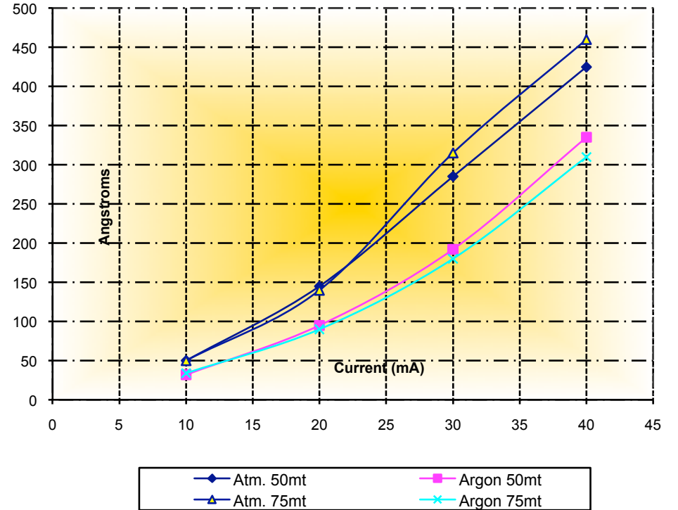
Deposition Rate Gold/Paladium Target 120 seconds
