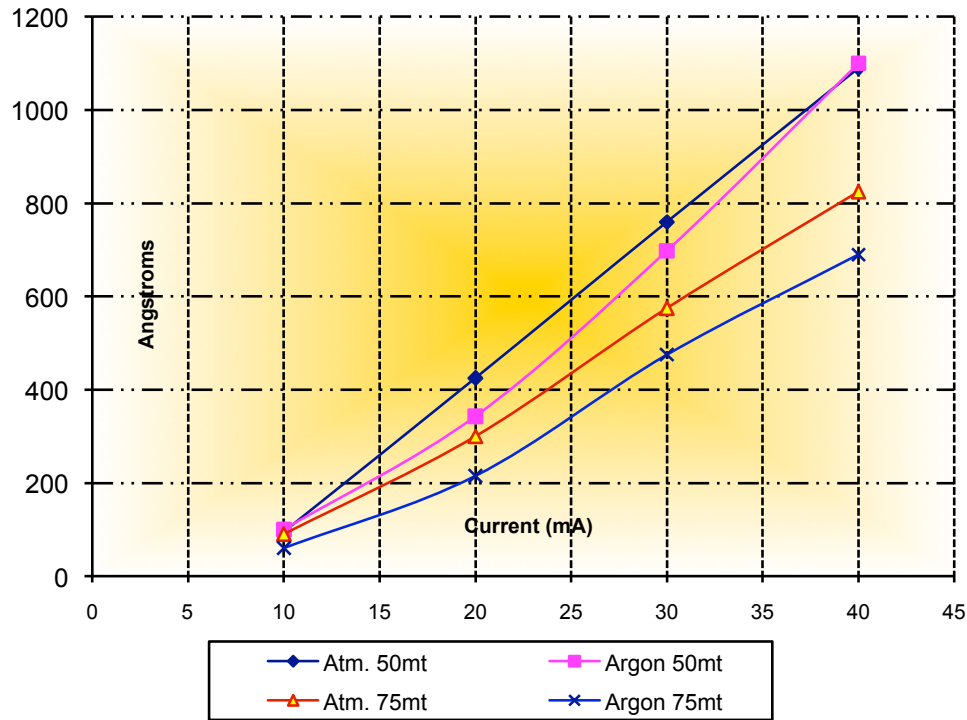
Deposition Rate Gold Target 120 seconds
